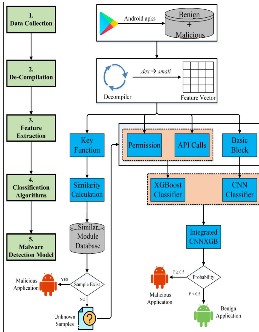
Fig 1: System architecture
