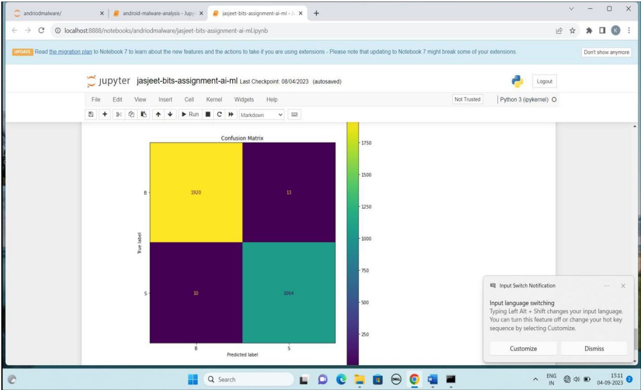
Fig 4: - Confusion matrix
