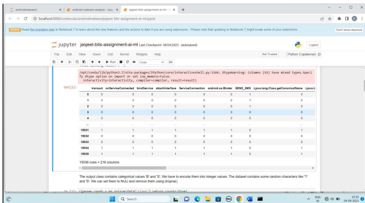
Fig 2: - sample dataset
